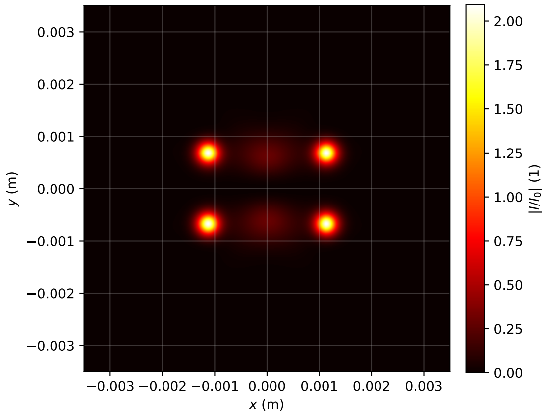
Intensity profile I(x, y, z = 2.149)/I_0 , P_{in}=4.0P_{cr} , artificial time
